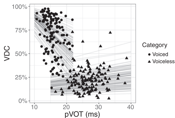
FIG. 5. Model-estimated cue values for pVOT (x axis) and VDC (y axis). Voicing category of the stop is represented by shape (points, voiced; triangles, voiceless). Points and lines represent the same values as in Figs. 3 and 4.
