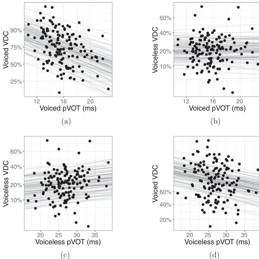
FIG. 6. Model-estimated cue values for pVOT ( x axis) and VDC ( y axis), comparing relationship between cues either within (left) or across (right) a given stop category. Points and lines represent the same values as in Figs. 3 and 4. pVOT in linear (ms) scale; VDC in logit-scaled probabilities to show differences at extreme probabilities (near 0% or 100%).
