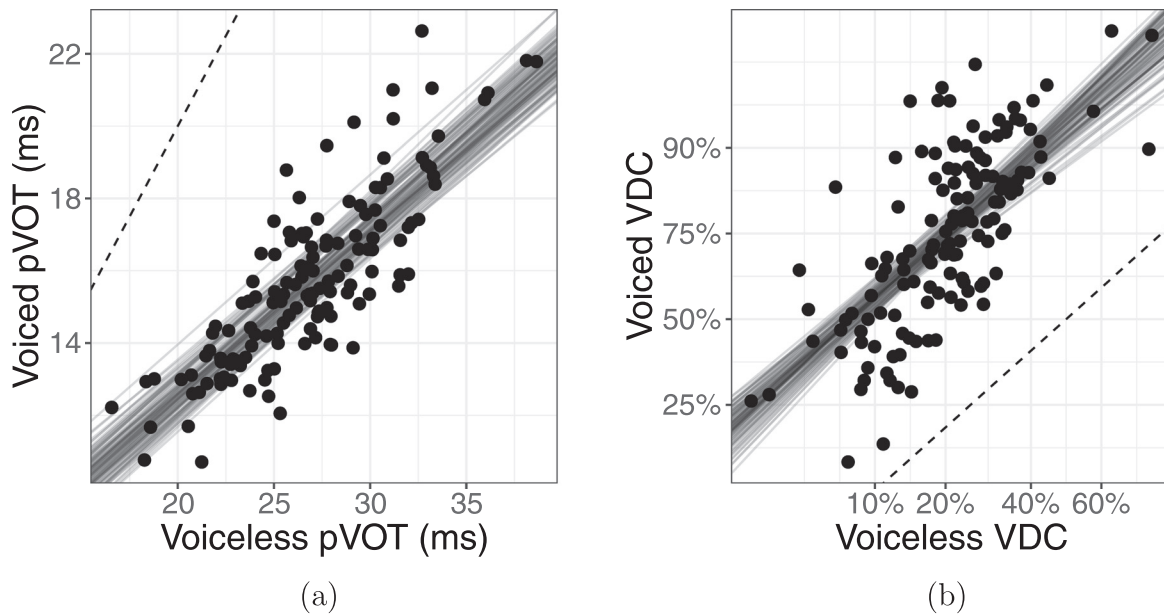
FIG. 3. Model-estimated cue values for pVOT (a) and VDC (b) for voiceless ( x axis) and voiced ( y axis) stops. One point is the posterior mean value for a particular speaker. Black lines are 100 lines of best fit drawn from the model posterior to show direction and uncertainty in the correlation. Dashed line is y = x , where the value for voiceless stops equals that for voiced stops. pVOT plot in linear (millisecond) scale; VDC plot is in logit-scaled probability scale to illustrate differences at extreme upper and lower probabilities.
