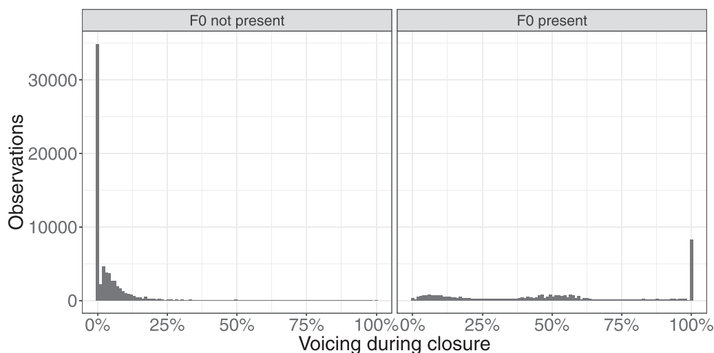
FIG. 2. Histograms showing the distribution of the percentage of voicing during closure by whether F_0 was also detected within the stop closure. One-hundred bins used within each histogram, meaning that each bar represents 1%.
