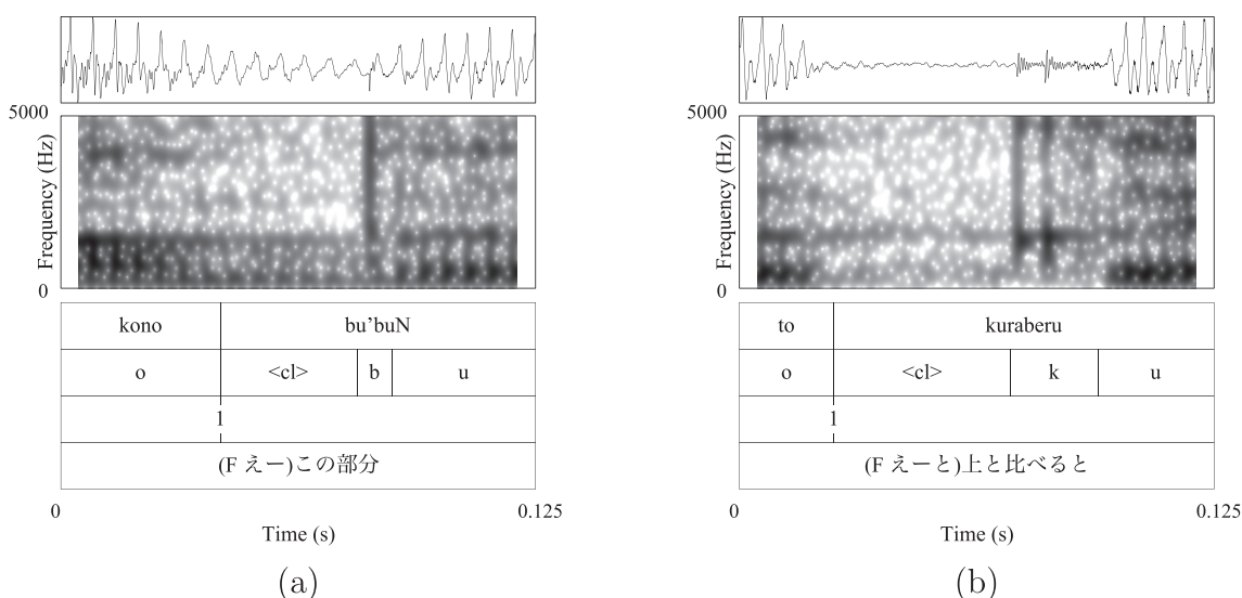
FIG. 1. Waveforms and accompanying annotations for phrase-internal stops realised with and without VDC [“kono bubun,” (a); “to kuraberu,” (b), respectively] produced by a female speaker taken from a 125 ms time window. Closure annotated as <c1>. Top tier represents word-level transcription, second tier contains phone and sub-phone annotations, third tier marks prosodic boundaries via Break Index, and fourth tier contains utterance transcription.
